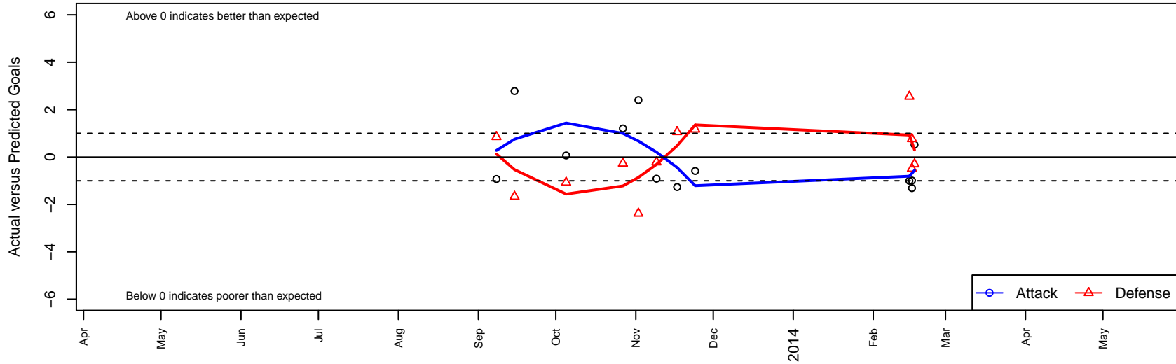
Palo Alto SC 97 Blue B96 Dots are actual minus expected GF (blue circles) and GA (red triangles). Blue line is smoothed change in attack strength. Red is smoothed change in defense strength.
